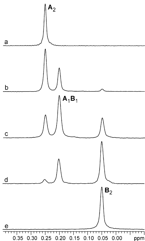
Figure 2. ^6\text{Li} NMR spectra of 0.10 M mixtures of [\text{}^6\text{Li}]\text{I} (A) and [\text{}^6\text{Li}]\text{II} (B) in 1.0 M TMEDA/toluene at -90\text{ }^\circ\text{C} . Key: (a) X_2 = 0.0 ; (b) X_2 = 0.23 ; (c) X_2 = 0.52 ; (d) X_2 = 0.79 ; (e) X_2 = 1.0 .
