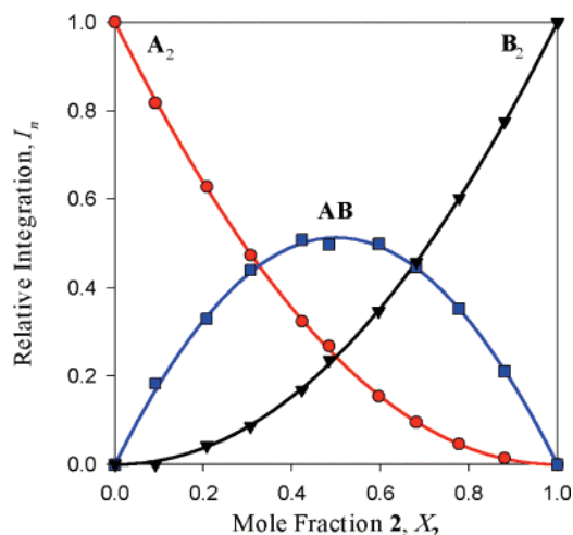
Figure 3. Job plot showing the relative integrations versus mole fraction of 2 for 0.10 M mixtures of enolates [\text{}^6\text{Li}]\text{I} (A) and [\text{}^6\text{Li}]\text{II} (B) in 1.0 M TMEDA/toluene at -90\text{ }^\circ\text{C} . From eqs 4–6: \phi_0 = 0.95 ; \phi_1 = 1.0 ; \phi_2 = 0.95 .
